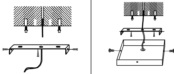
Ceiling installation diagram
